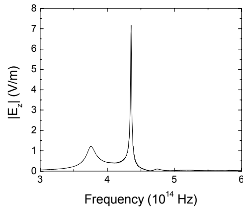
Figure 4. Fourier Transform of the time domain E_z signal at location 1.
