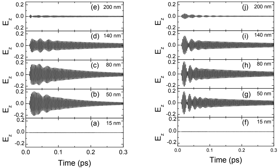
Figure 7. Time dependence of the E_z field at location 1 for various particle-film separations. The height of the center of the particle is indicated in each graph. Graphs (a)-(e) correspond to AR = 2.5, and graphs (f)-(j) correspond to AR = 3.5.
