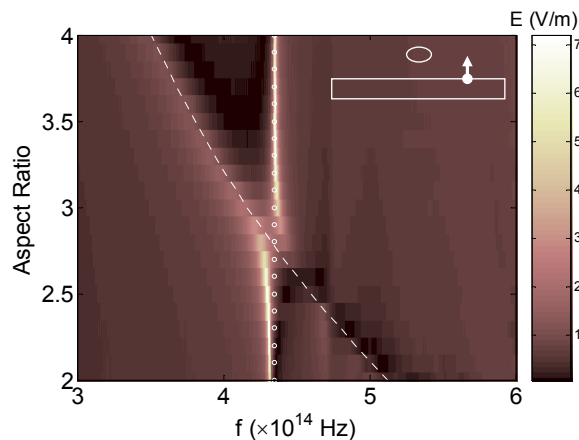
Figure 6. Electric field strength of oscillations in the frequency range 3 \times 10^{14} Hz to 6 \times 10^{14} Hz at location 1 as measured in the simulations. The color represents the magnitude of the relevant component of the electric field.
