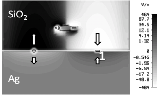
Figure 2. E_z fields at y = 0 at a frequency of 4.35 \times 10^{14} Hz. The + and - signs schematically indicate the location of charges and the arrows indicate the directions of the fields.
