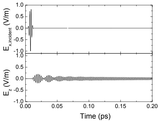
Figure 3. Top: excitation signal monitored at the port. Bottom: Time evolution of the E_z field at location 1.
