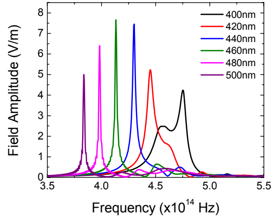
Figure 5. E_z at location 1 for L_x ranging from 400 nm to 500 nm, at an aspect ratio of 2.5.
