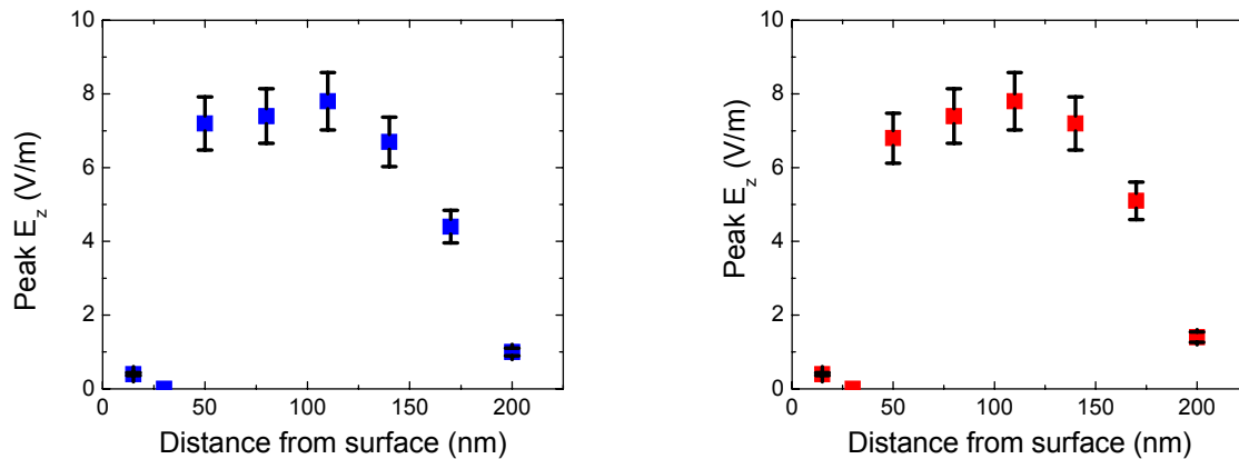
Figure 8. Peak E_z value of the surface plasmon resonance for as a function of particle-film separation, showing (a) results for AR = 2.5, and (b) results for AR = 3.5. The error bars are representative of the inaccuracy of the calculations as described in section 2.
